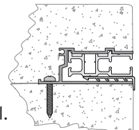
Deck-on-deck with Dual Race track channel
