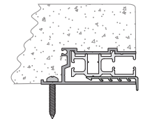
Raised Dual Race track channel
